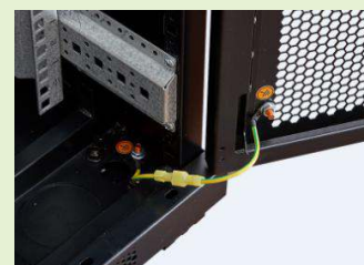
Ground wire
